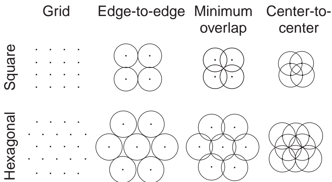
Figure 7.2: Coverage patterns
